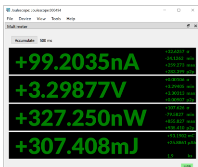
Multimeter view
