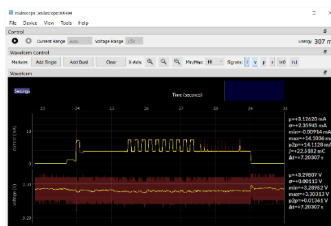
Oscilloscope view
