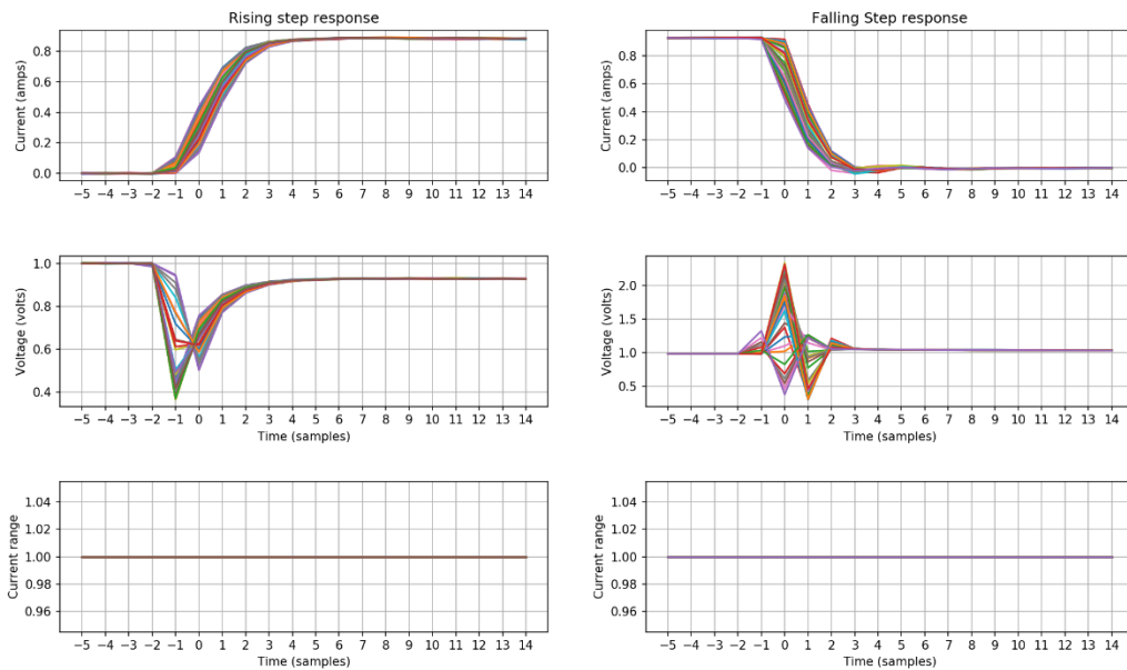
Figure 2: Step response with fixed 2A range
